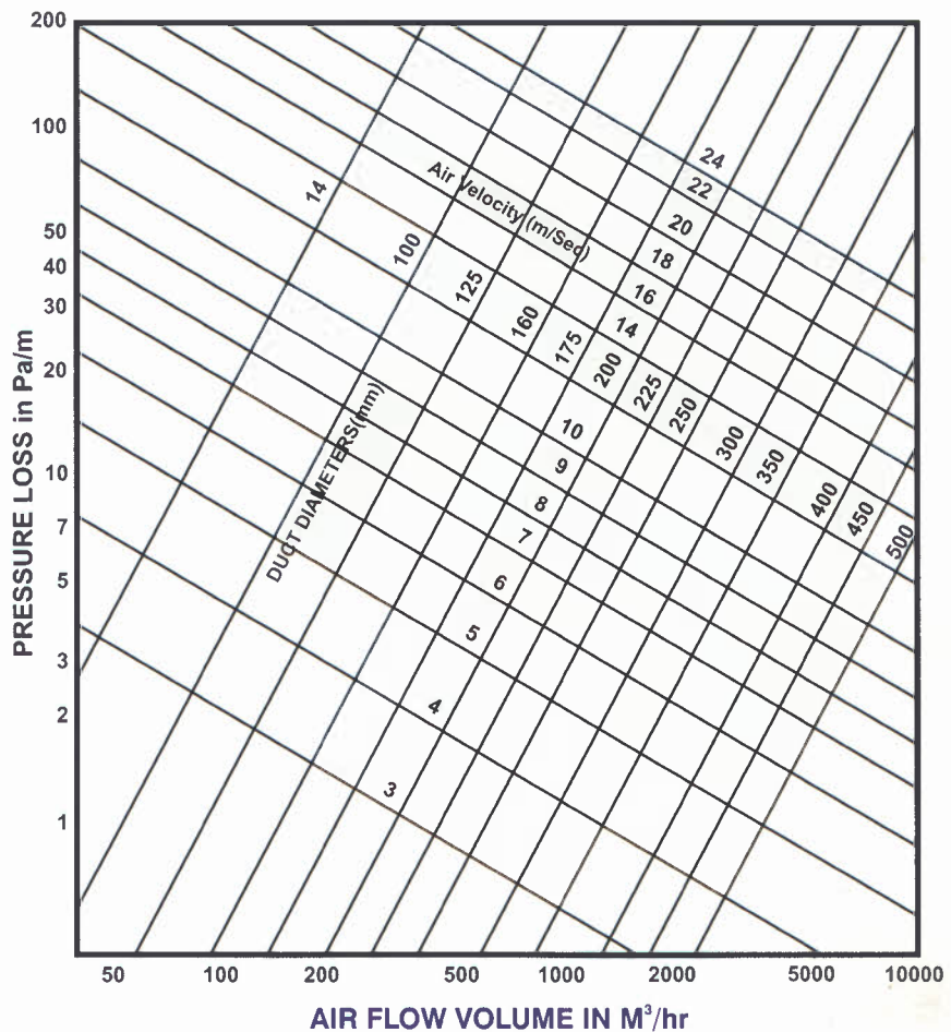
Pressure loss diagram
